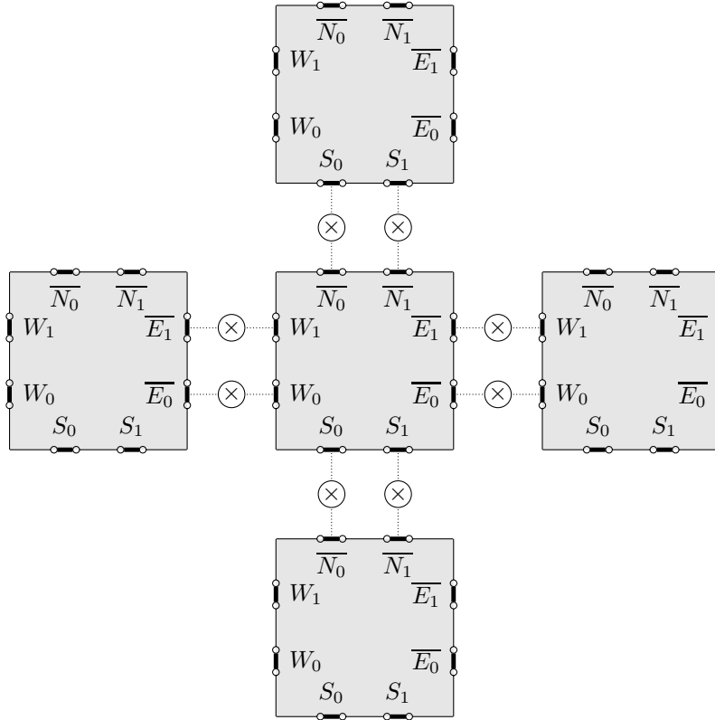
FIGURE 14. Second step in global construction – the graph G^2 (for two colors c_0 and c_1 )
