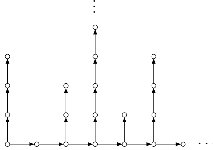
FIGURE 2. A comb with one infinite tooth, the only spine is the horizontal ray.
