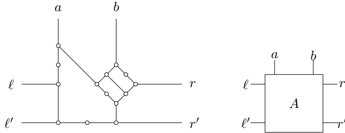
FIGURE 7. Graph G from the proof of Thm. 3.4
