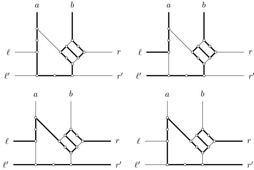
FIGURE 9. Paths through the graph A
