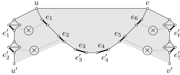
FIGURE 7. Graph G from the proof of Thm. 3.4
