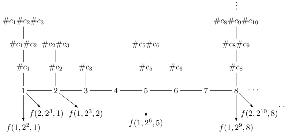
FIGURE 15. A graph \overline{G(M_1, M_2)} with M_1 \notin \text{COF}
