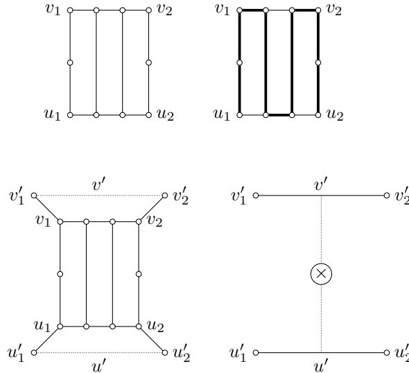
FIGURE 4. The graph X , its use and abbreviation
