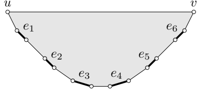
FIGURE 6. Graph G_0 from the proof of Thm. 3.4
