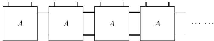
FIGURE 10. The infinite graph L
