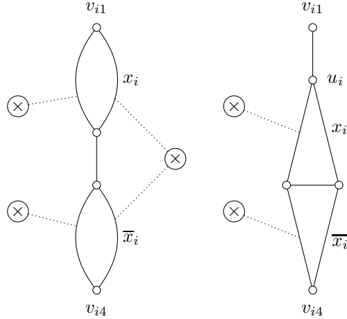
FIGURE 5. Simplification of the graph from [13]
