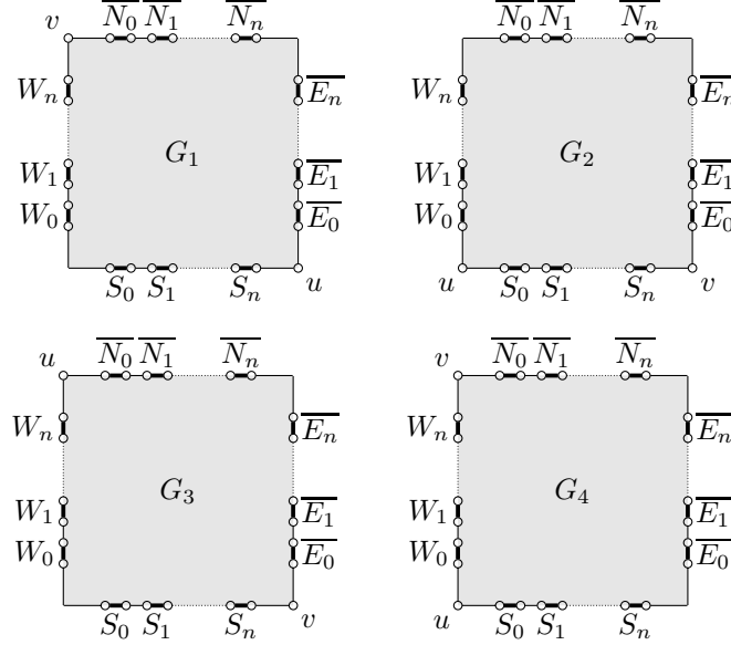
FIGURE 12. The graphs G_x
