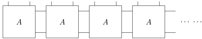
FIGURE 9. Paths through the graph A
