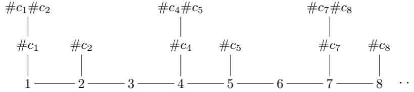
FIGURE 15. A graph \overline{G(M_1, M_2)} with M_1 \notin \text{COF}
